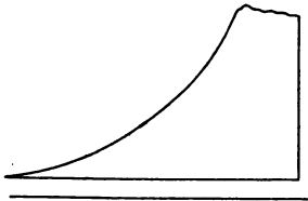
FIG. 65.—Mechanically operated inlet valve opened at end of stroke.
